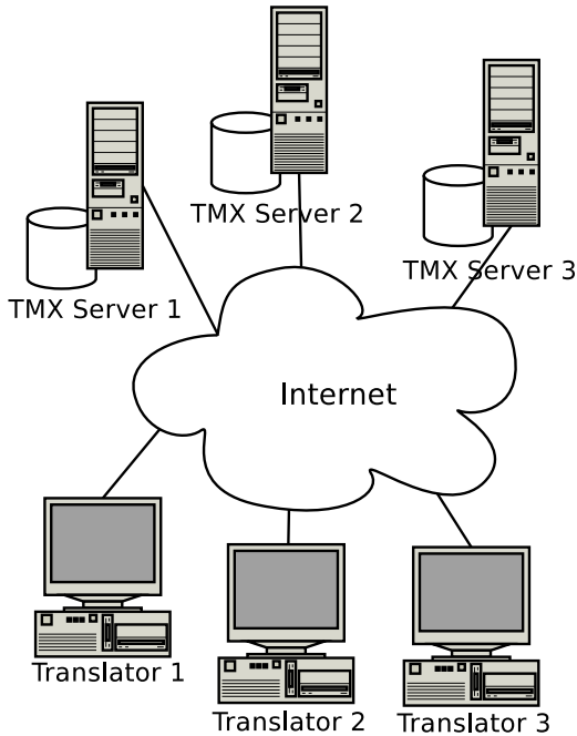
Figure 2: Client/server architecture
