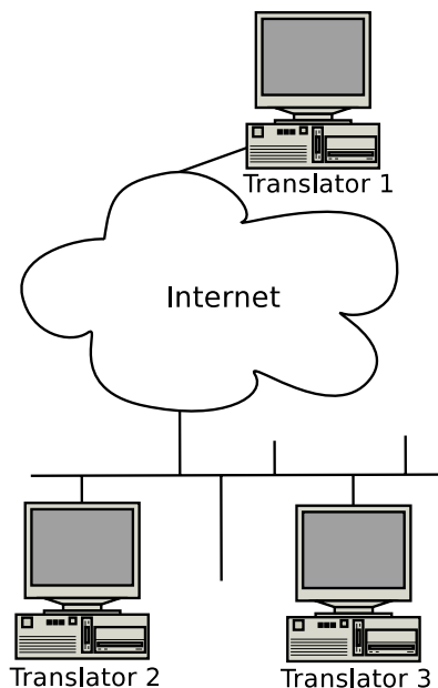
Figure 1: Peer-to-peer architecture
